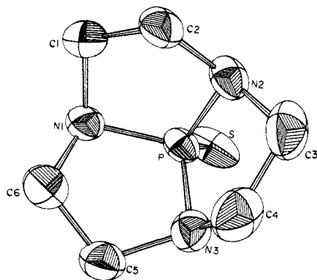
Figure 1. Computer drawing of molecular structure of 3 .
